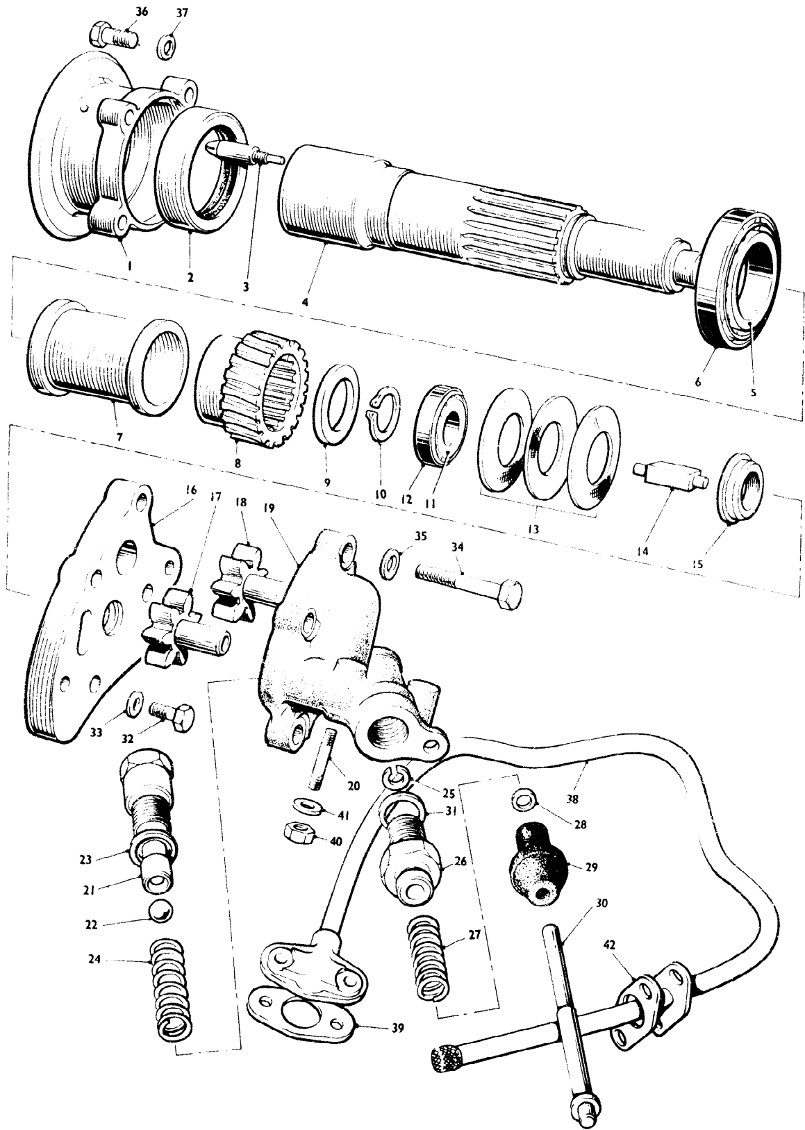
SERVO DRIVE
