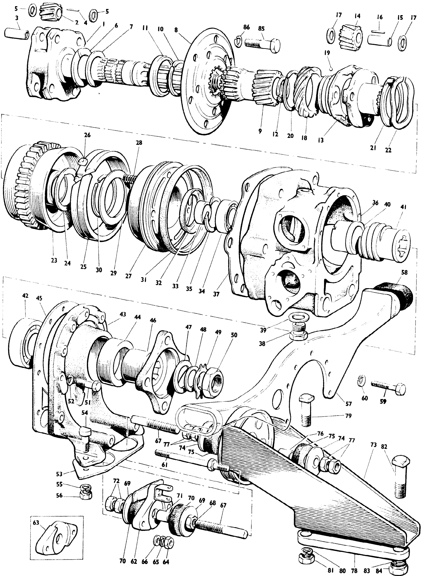
OUTPUT SHAFT REVERSE ASSEMBLY
