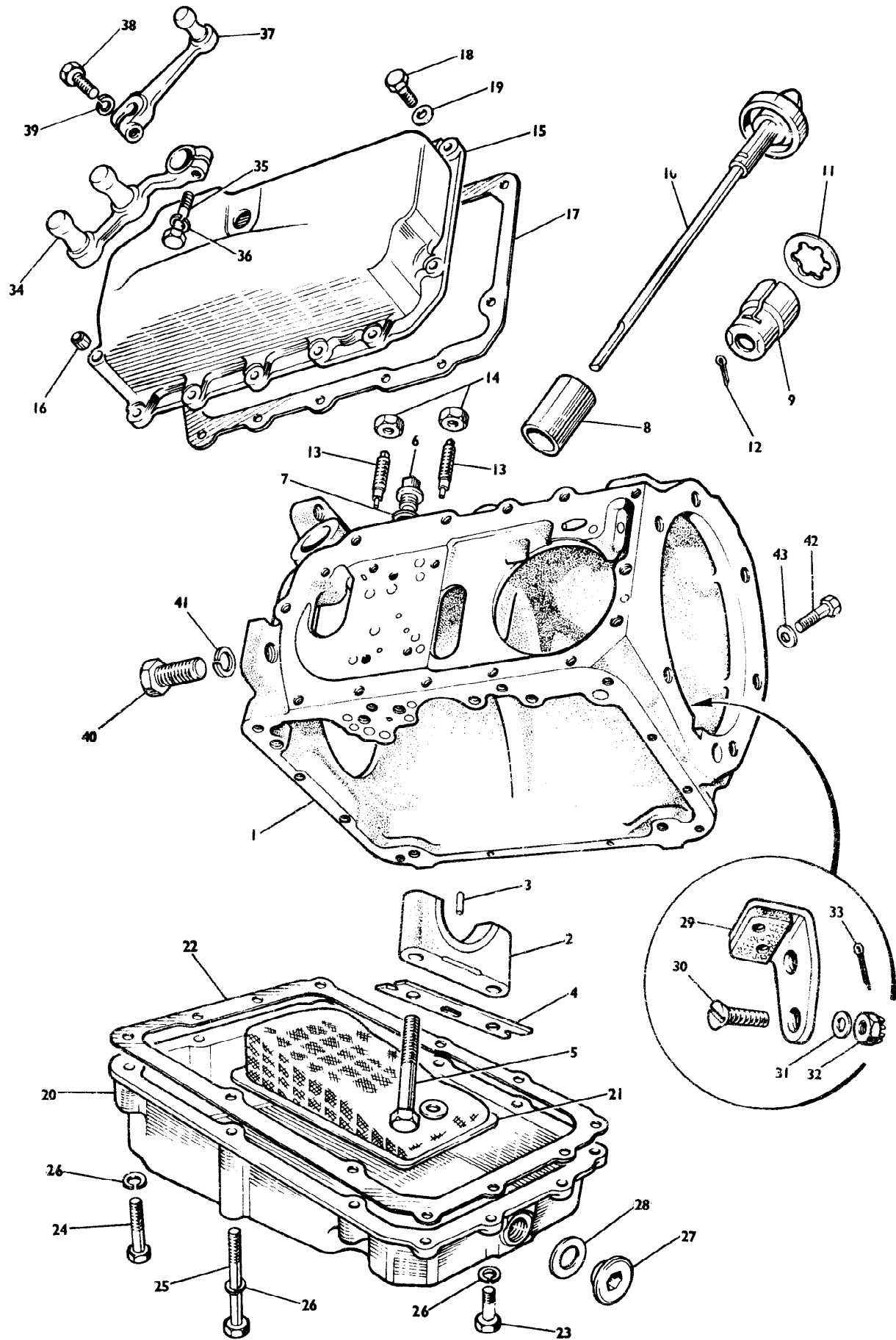
GEARBOX CASING
