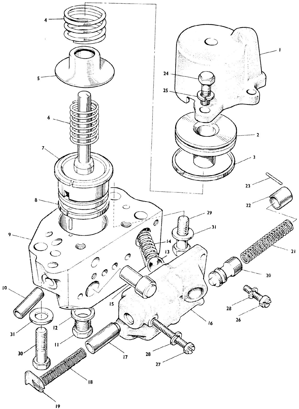
FRONT SERVO
